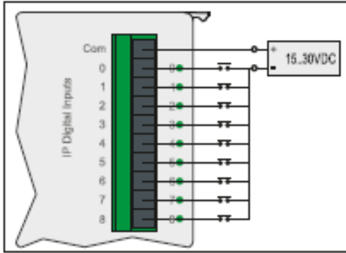
npn connection
