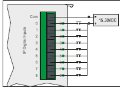
pnp connection
