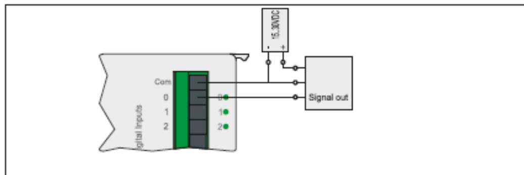
Encoder Connection
