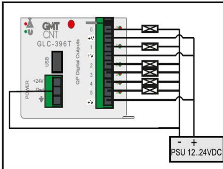
Hardware revision 07 and higher connection diagram
