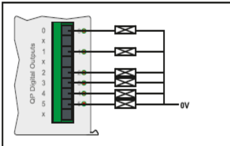
Connection diagram
