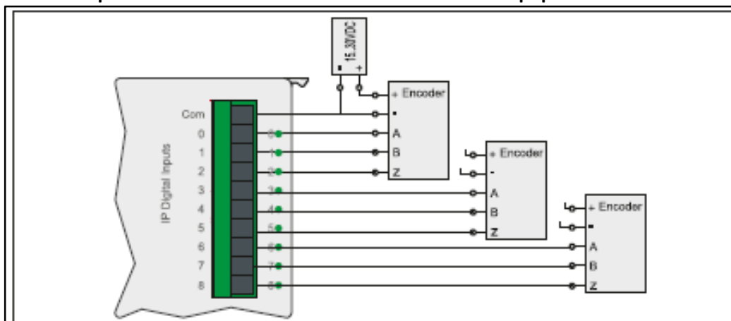
Encoder Connection
